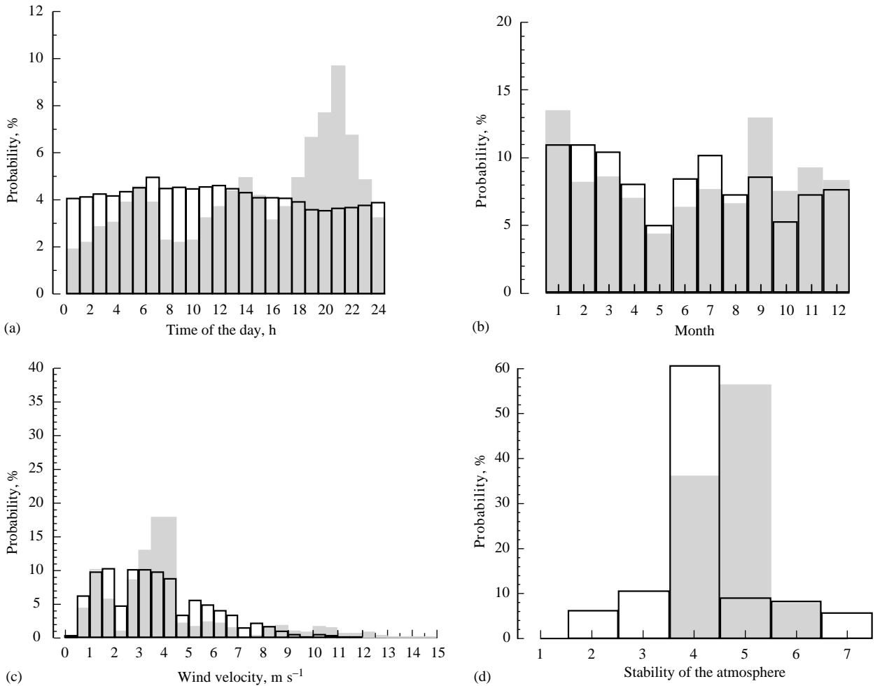
Fig. 7. Comparison of the probability for West wind (separation distance East) for the entire two-year period (□) and the probability of odour sensation (■) at the separation distance calculated for the odour impact criterion G-PURE defined by an odour concentration threshold of 1 OU m -3 and the probability of the threshold exceedance of 3% for the hour of the day (a), for the months of the year (b), for wind velocity (c), and for the stability of the atmosphere (d)
